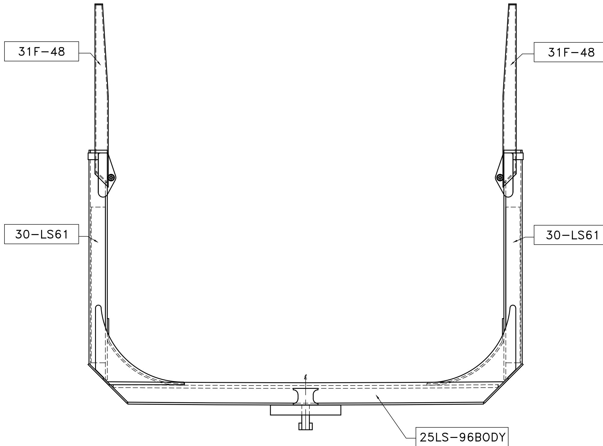
9'-6" SOLID BUNK BODY 61" STAKES 48" EXTENSIONS LONG LOGGER TRUCK
