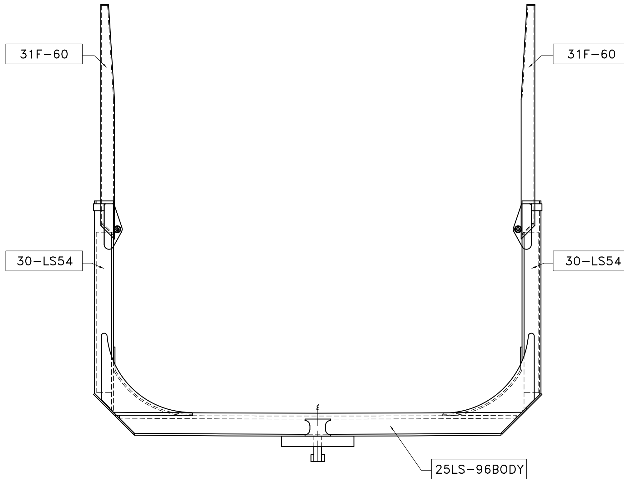
9'-6" SOLID BUNK BODY 54" STAKES 60" EXTENSIONS LONG LOGGER TRAILER
