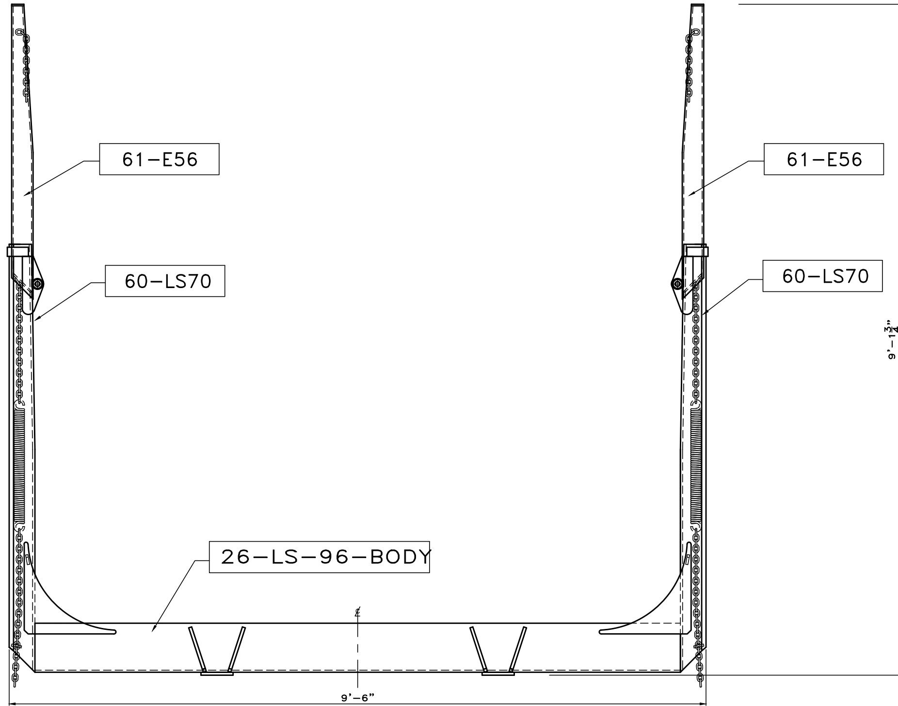
60BT-96-70-56 9'-6" SOLID BUNK BODY 70" STAKES 56" EXTENSIONS B TRAIN OR HAYRACK BELLY
